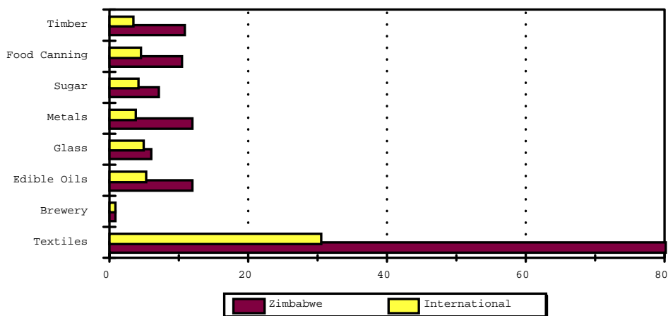
Figure 4: Comparison of the country's industrial energy intensities to international trends in GJ/unit of production.
